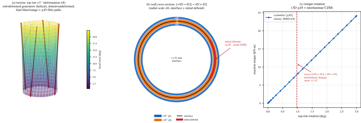
Figure 3: CFRP drive shaft under torsion. (a) 3-D twist of the [\pm 45] tube (deformation \times 8 ; red = deformed generators turned helical, dotted = undeformed); (b) wall cross-section [+45/-45 \parallel -45/+45] (radial scale exaggerated) with the interlaminar interface and initial debond patch; (c) torque-rotation of the 3-D \pm 45 laminate with interlaminar cohesive zones.
