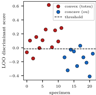
(a) scale-invariant signature AUROC 0.91, p=0.005
