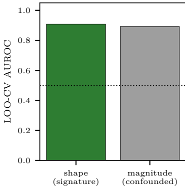
(b) the defect SIGNATURE discriminates, not just loading amplitude
