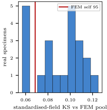
(c) real data is OOD vs FEM (77)
