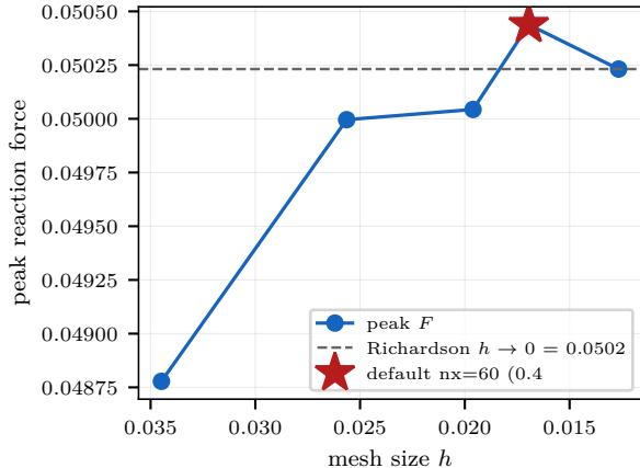
(b) QoI mesh convergence (load=0.10, \ell frozen)
