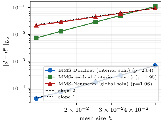
(a) MMS convergence — damage operator
