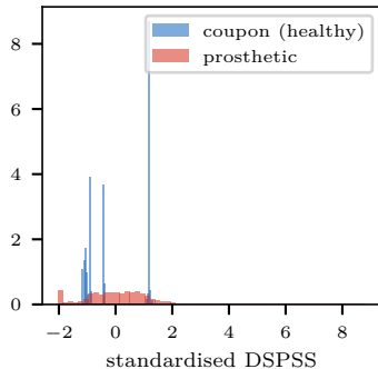
(b) domain gap KS=0.29
