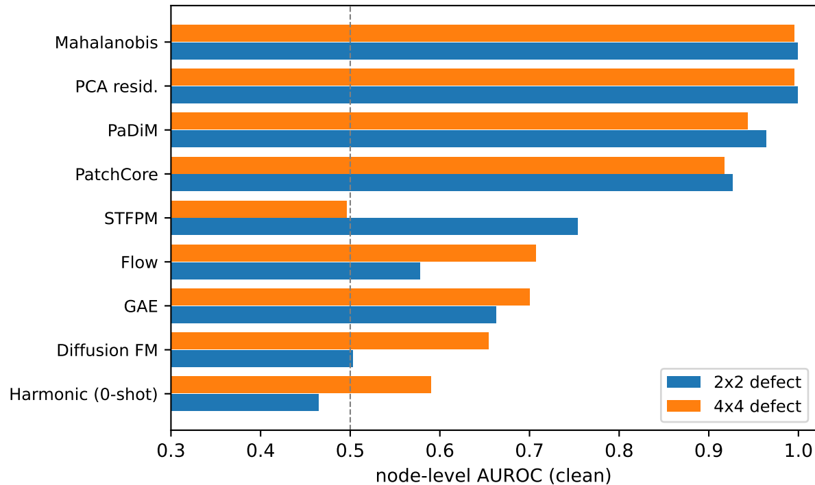
(a) Simple node-space statistics beat deep methods
