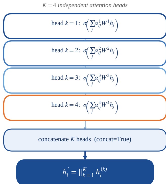
(C) Multi-head update h'_i
