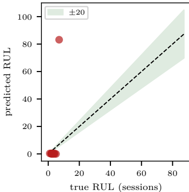
(b) LOCO RUL: \alpha-\lambda=0
