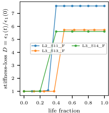
(a) real run-to-failure trajectories (REAL NASA)
