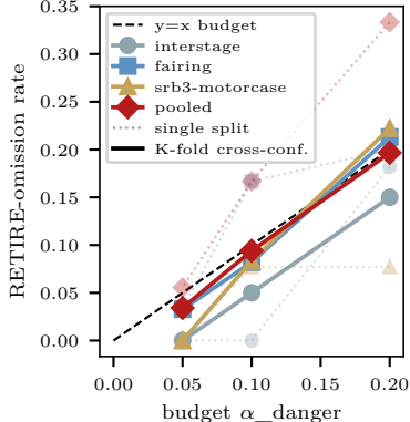
(c) dangerous-omission: cross-conformal fix (on/below diagonal = within budget)
