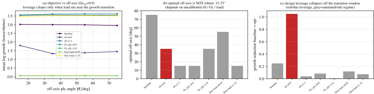
Figure 12: Stage 5 robustness. Perturbing the uncalibrated phase-field constants ( \ell , G_c^{\text{ply}} ) and the fleet load: (a) the objective has off-axis leverage only near the growth transition; (b) the optimal off-axis angle spans 15°–75° (not robust); (c) the design improvement collapses once the constants push the operating point off the transition window.
