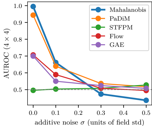
(b) Collapse by \sigma = 0.1 : per-measurement SNR limit
