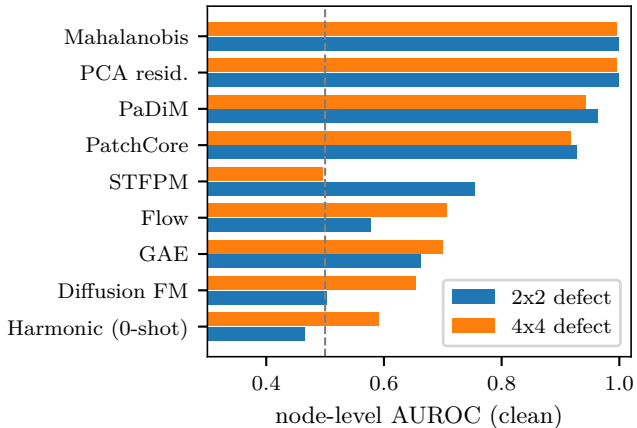
(a) Node-space statistics beat deep methods
