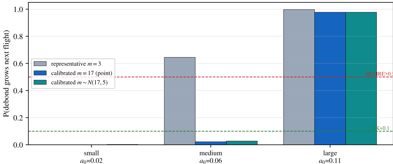
Stage-3 fairing prognosis: representative vs REAL-data-calibrated Paris exponent (4TU DCB mode-I, m \approx 17 not 3; LOSO fails \Rightarrow propagate the population spread)
