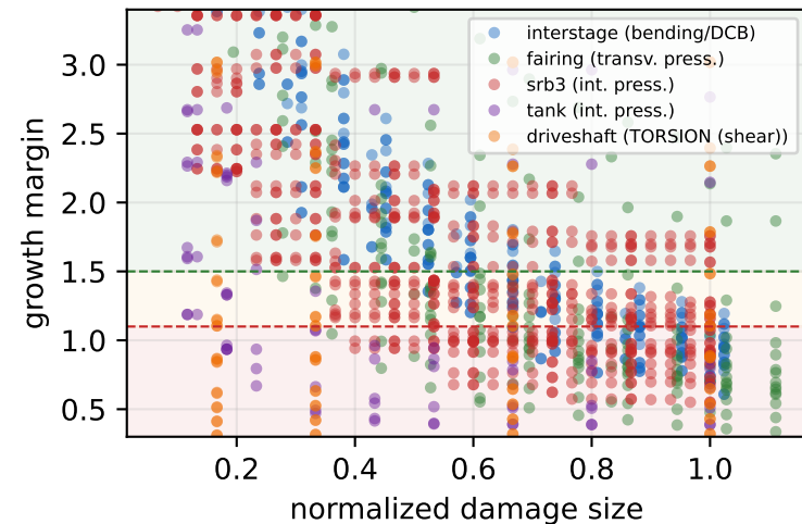
(a) 5 structures, ALL real FEM (incl. TORSION)
