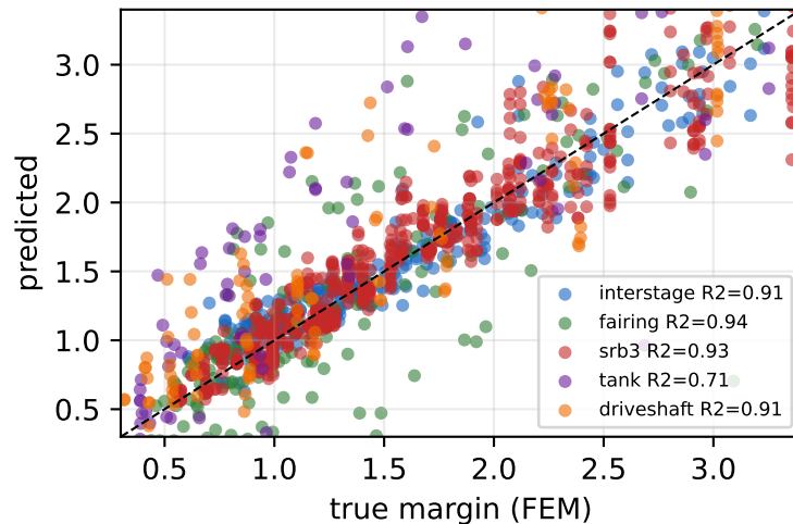
(b) single structure-agnostic surrogate R^2=0.94 , dangerous-miss=0.011
