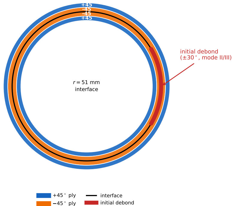
(b) wall cross-section: [+45/-45 \parallel -45/+45] (radial scale \times 6 ; interface + initial debond)
