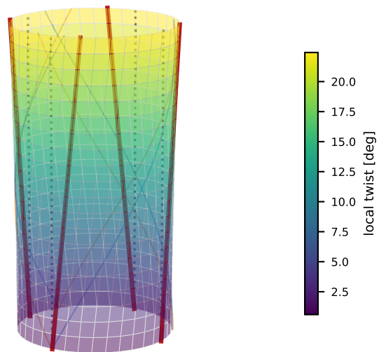
(a) torsion: top rim +3^\circ (deformation \times 8 ) red=deformed generators (helical), dotted=undeformed; faint blue/orange = \pm 45 fibre paths
