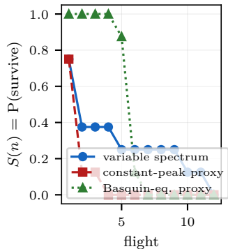
(b) survival: spectrum vs proxy
