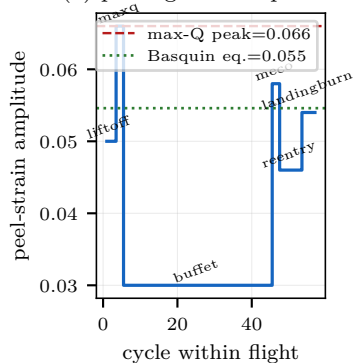
(a) per-flight load spectrum
