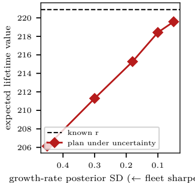
(c) resolving growth-rate uncertainty buys lifetime value
