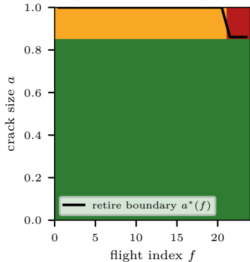
(a) optimal policy map (green FLY / amber REPAIR / red RETIRE)
