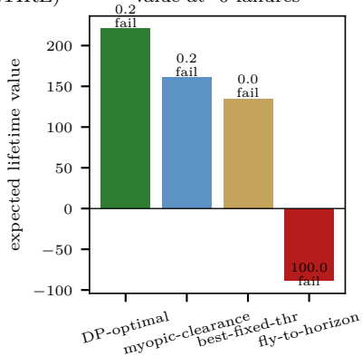
(b) DP-optimal extracts the most value at 0 failures
