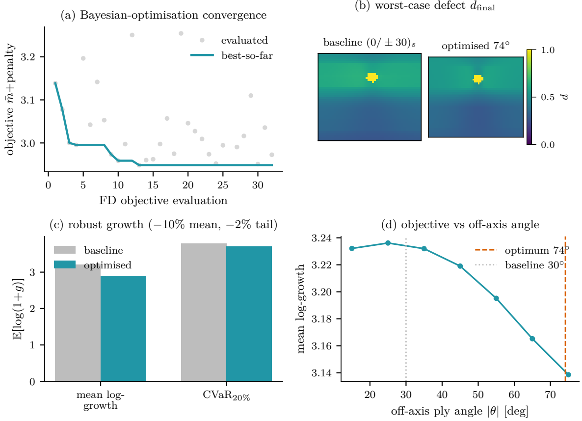
Figure 10: Stage 5. (a) BO convergence; (b) worst-case damage, baseline vs. optimised layup; (c) mean/CVaR growth; (d) objective vs. off-axis angle.
