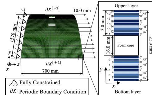
FEM boundary conditions & hole geometry.
