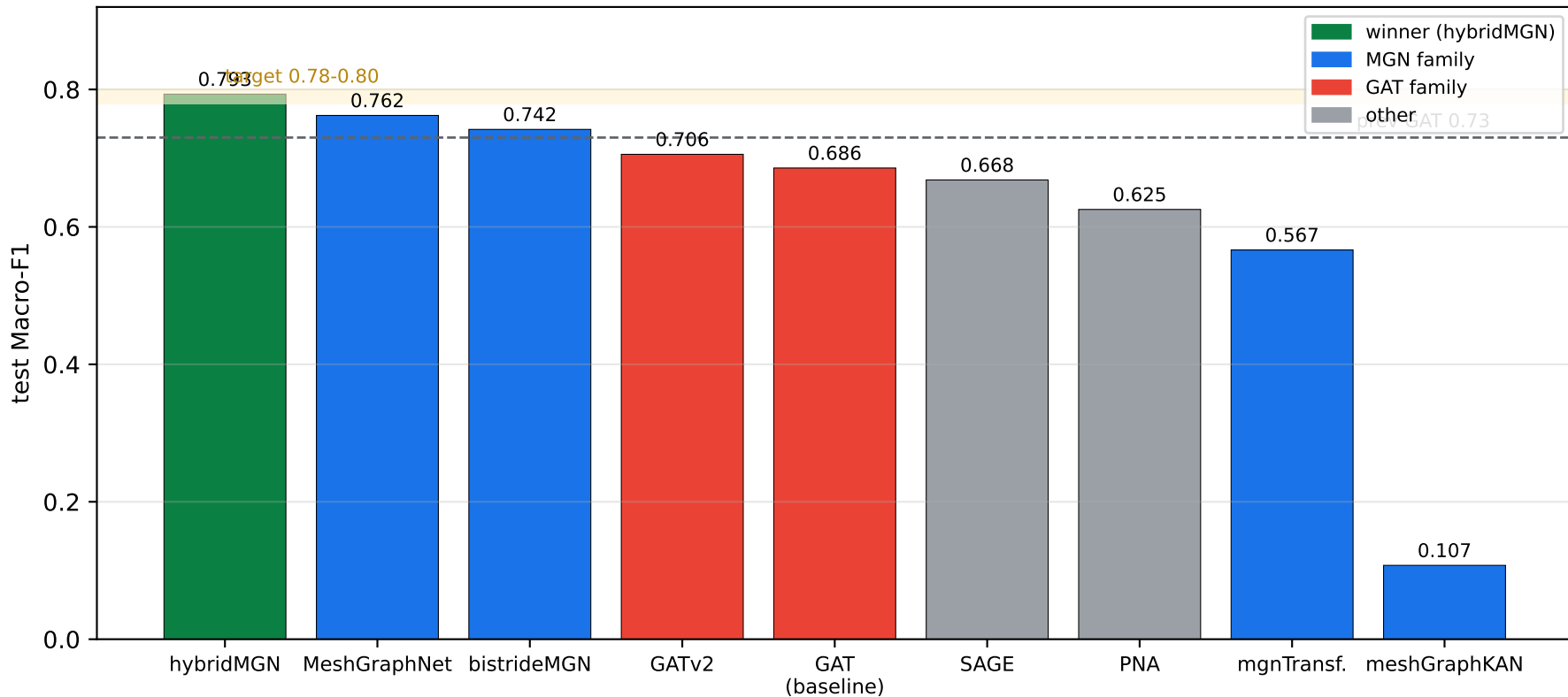
Architecture sweep (19-class CFRP defect, fix=no-logit-adjust + class-freq sampler)
