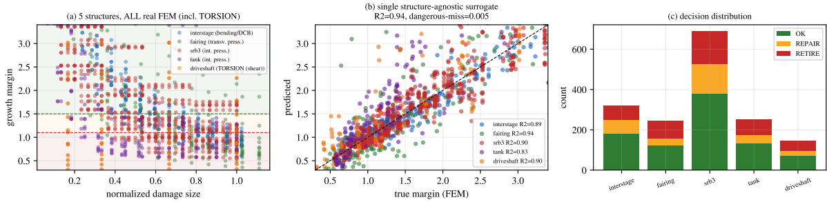
Figure 4: Structure-agnostic margin surrogate over 1,499 real-FEM states across five structures. (a) growth margin vs. damage size; (b) single surrogate in-distribution ( R^2 = 0.94 , dangerous-miss=0.005); (c) decision distribution. A leave-one-load-mode-out hold-out of the torsion drive shaft does not extrapolate — load mode, unlike geometry, is a genuine generalisation boundary.
