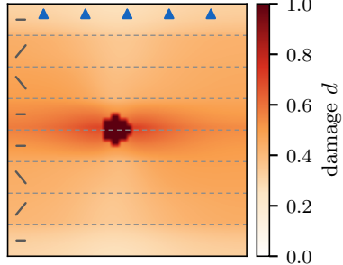
(c) interface delamination, load 0.115
