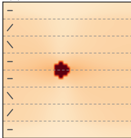
(b) sub-critical, load 0.085
