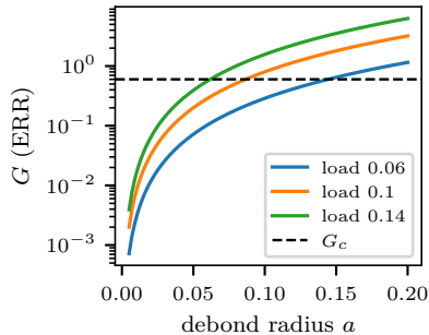
(a) interfacial driving force
