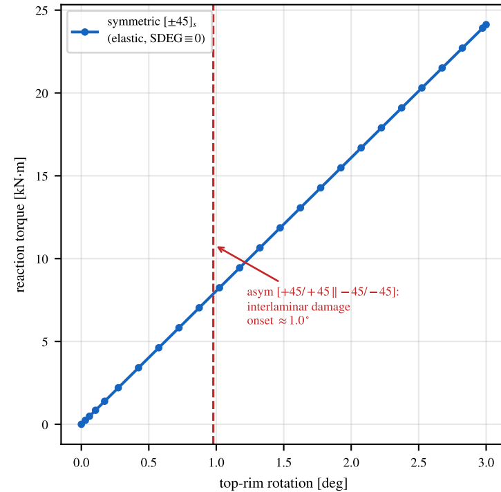
(c) torque-rotation (3D \pm 45 + interlaminar CZM)
