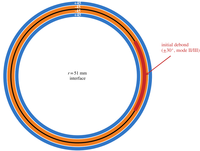
(b) wall cross-section: [+45/-45 \parallel -45/+45] (radial scale \times 6 ; interface + initial debond)
