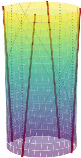
(a) torsion: top rim +3^\circ (deformation \times 8 ) red=deformed generators (helical), dotted=undeformed; faint blue/orange = \pm 45 fibre paths
