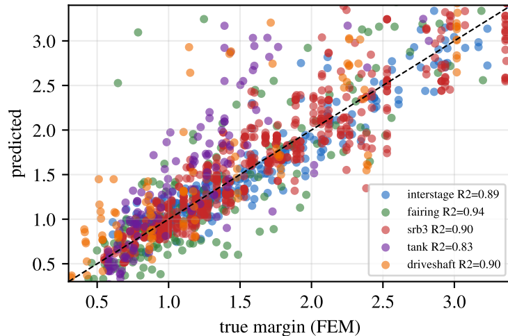
(b) single structure-agnostic surrogate R^2=0.94 , dangerous-miss=0.005
