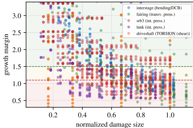
(a) 5 structures, ALL real FEM (incl. TORSION)
