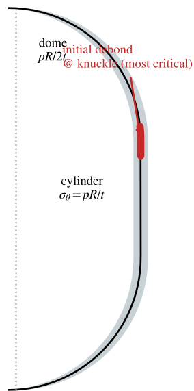
(b) meridional section: cyl \rightarrow knuckle \rightarrow dome, mid-wall interlaminar interface + debond
