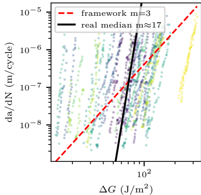
(a) real CFRP da/dN - \Delta G (steeper than m=3 ) (b) real m \gg 3 (fibre-bridging spread)
