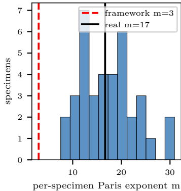
(a) real CFRP da/dN - \Delta G (steeper than m=3 ) (b) real m \gg 3 (fibre-bridging spread)
