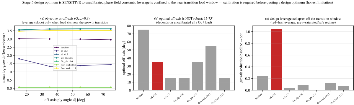
Figure 12: Stage 5 robustness. Perturbing the uncalibrated phase-field constants ( \ell , G_c^{\text{ply}} ) and the fleet load: (a) the objective has off-axis leverage only near the growth transition; (b) the optimal off-axis angle spans 15°–75° (not robust); (c) the design improvement collapses once the constants push the operating point off the transition window.
