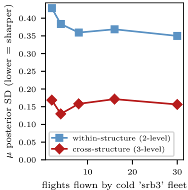
(b) cold-start learning curve (3-level sharper with less data)
