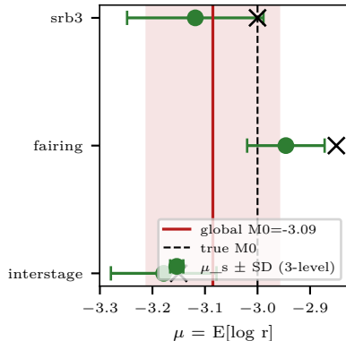
(c) recovered structures + global ( \times = truth)
