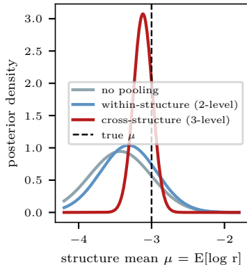
(a) cold-start 'srb3' \mu posterior (3-level sharpest: \times 2.96 vs 2-level)
