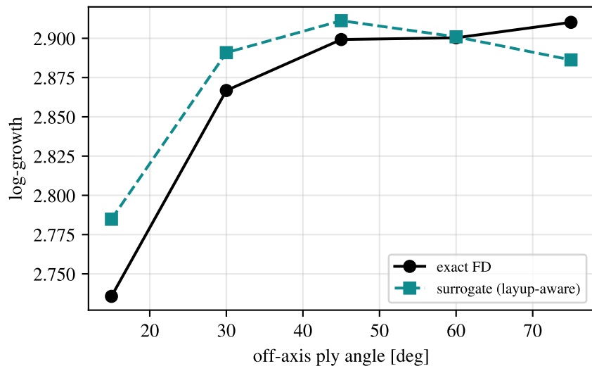
(b) captures the design dependence (the shipped FNO is layup-blind)
