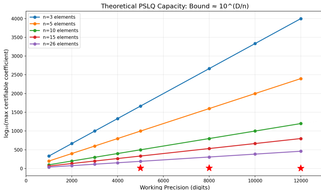
Figure 3: Theoretical PSLQ capacity: for a basis of n elements at D -digit precision, the maximum certifiable coefficient bound is approximately 10^{D/n} . Red stars mark our actual tests. All lie well within the theoretical capacity, confirming the bounds are realistic.
