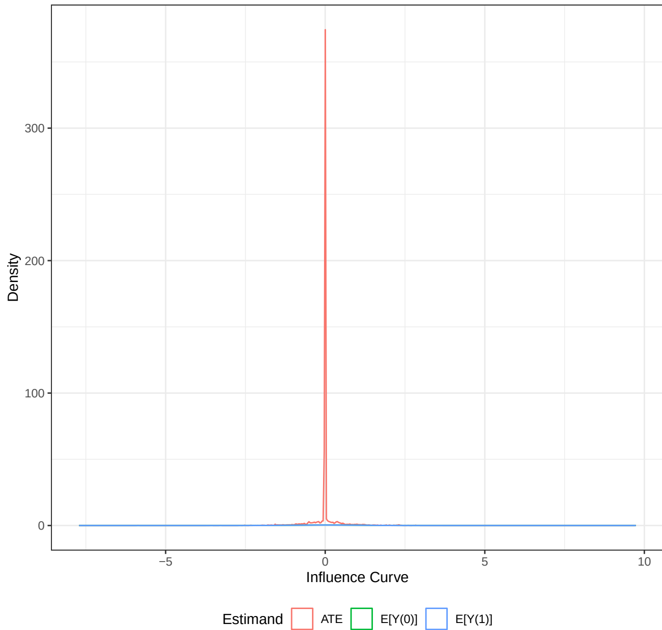
Influence Curve Distribution
