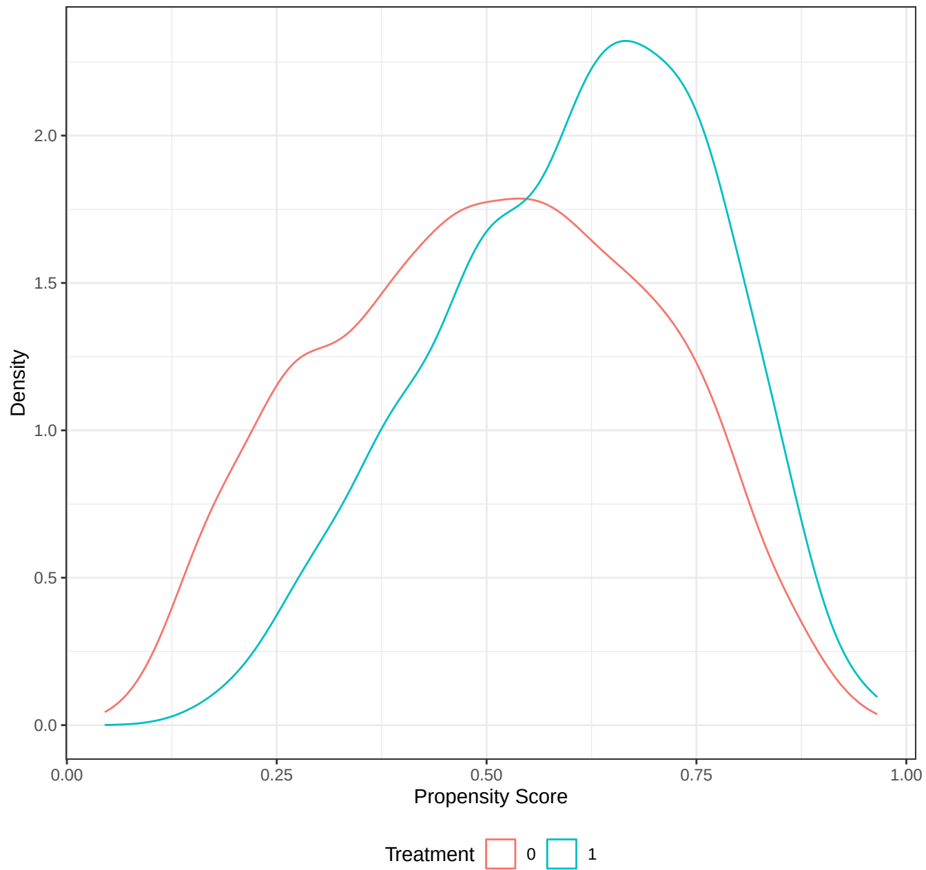
Treatment Propensity Score Distribution
