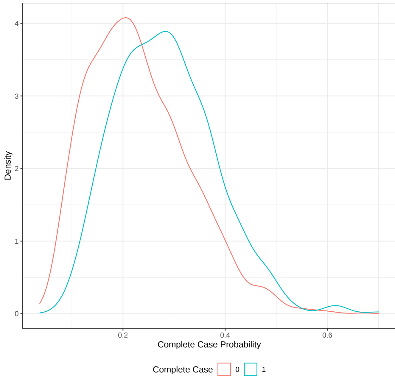
Complete Case Probability Distribution
