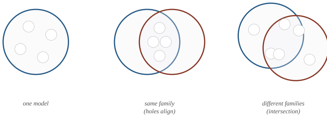
Figure 1. Hole-sets. Same-family slices leave holes aligned. Different-family slices shrink the residual intersection. Schematic, not a measured Venn.
