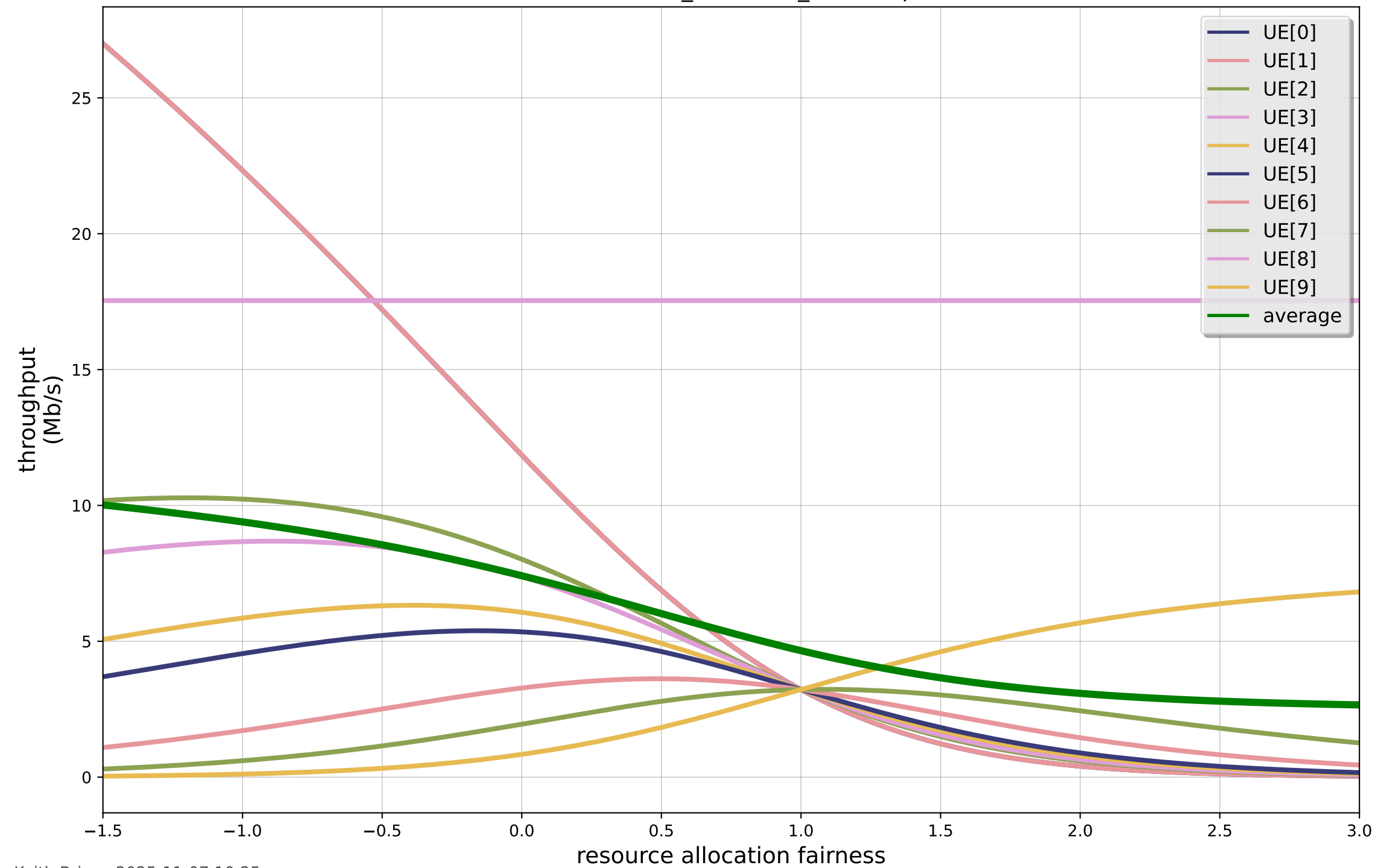
CRRM resource allocation n_{\text{cells}}=7 n_{\text{ues}}=10 p = -1.5, \dots, 3.0
