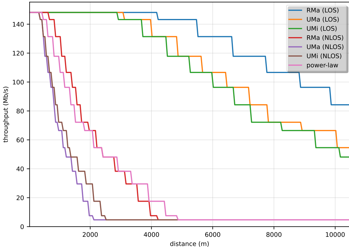
Throughput vs. distance by pathloss model
