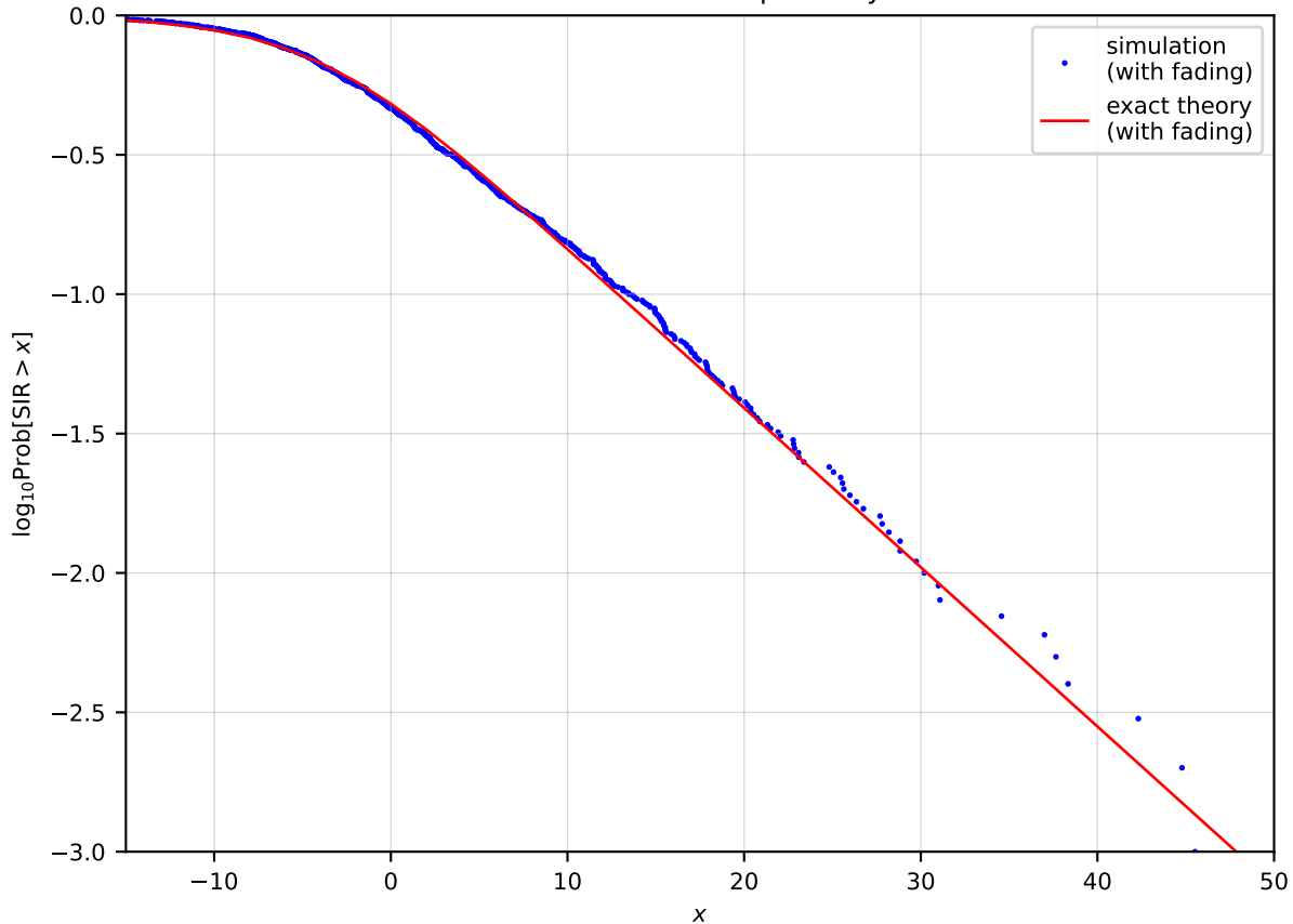
SIR distributions as computed by CRRM
