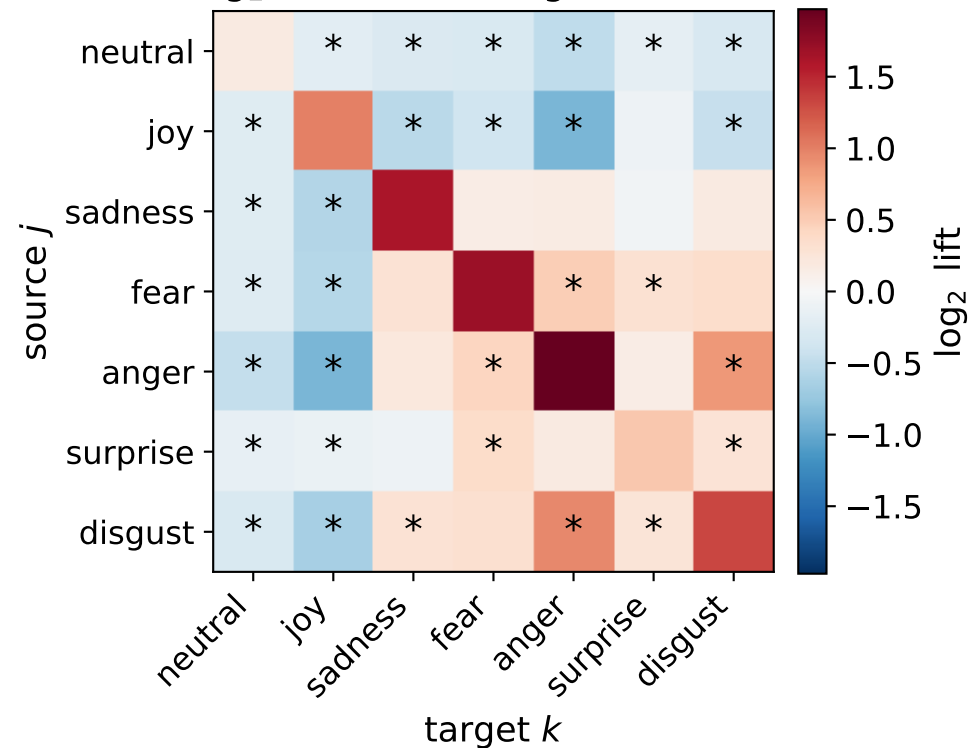
(a) \log_2 lift, BH-FDR-significant marked
