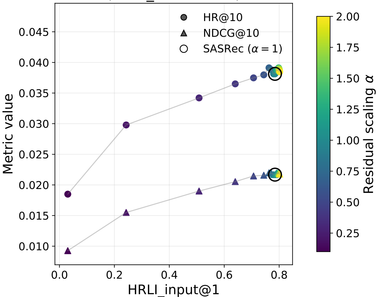
Beauty: Accuracy vs. HRLI_input@1 (filter_seen=True)
