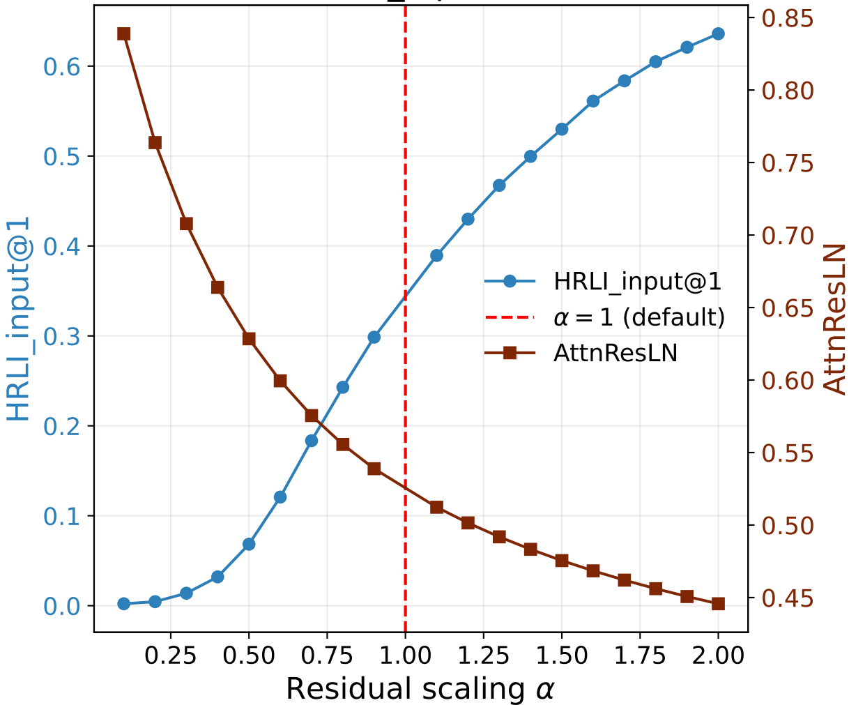
BeerAdvocate: HRLI_input@1 vs. AttnResLN
