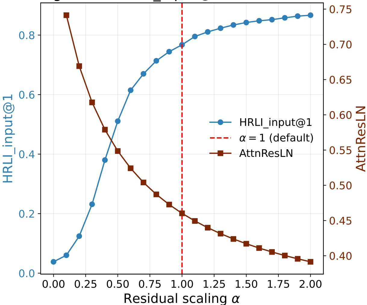
Diginetica: HRLI_input@1 vs. AttnResLN
