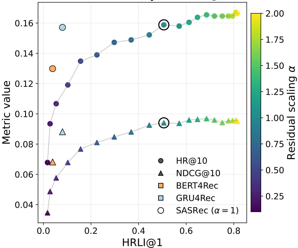
ML-1M: Accuracy vs. HRLI@1
