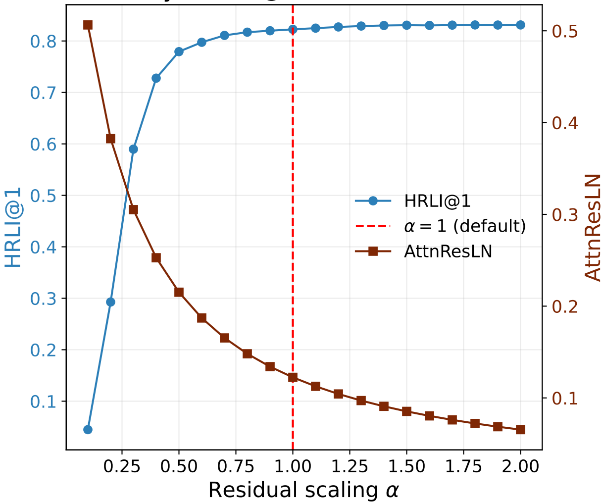
Toys: HRLI@1 vs. AttnResLN
