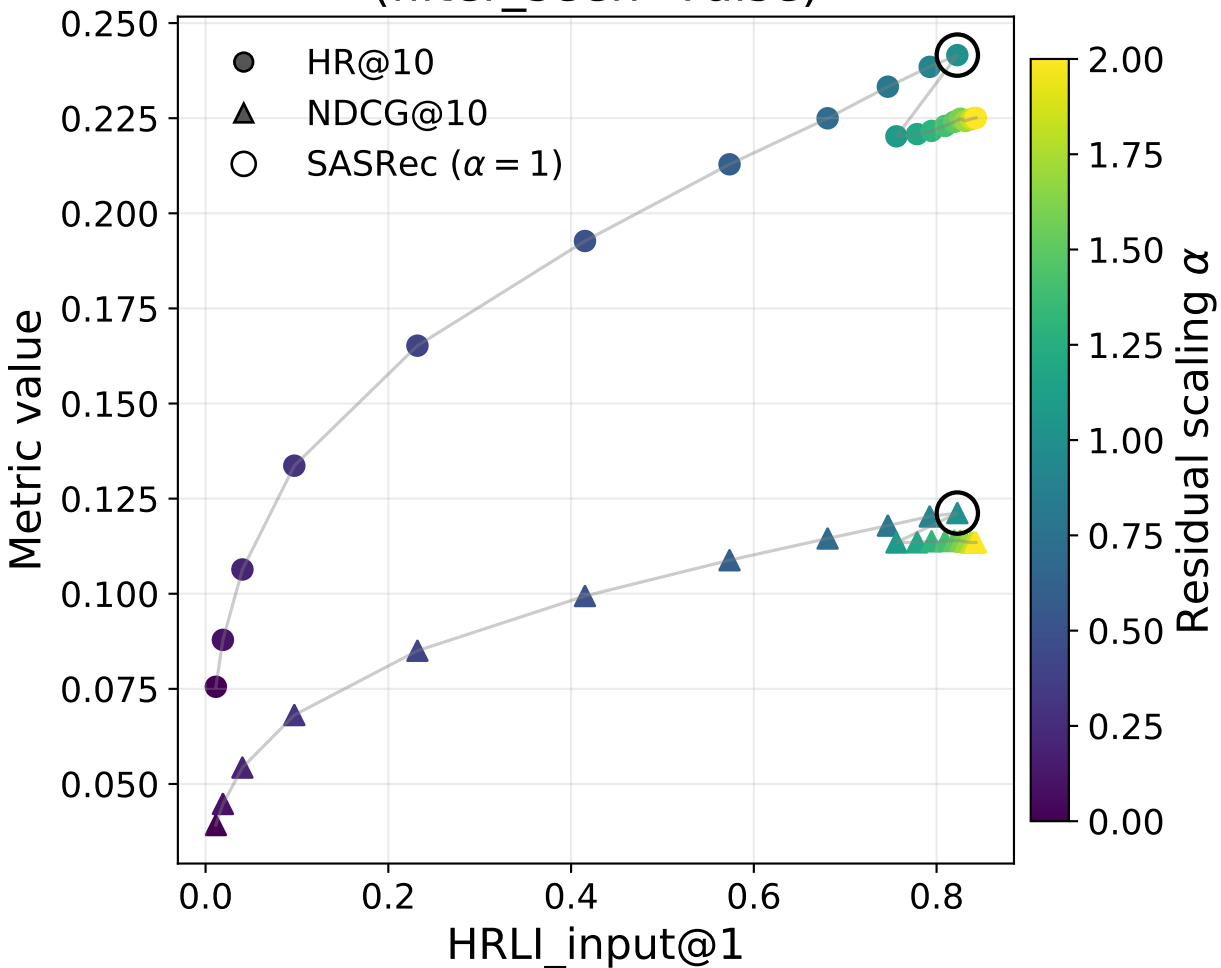
Zvuk: Accuracy vs. HRLI_input@1 (filter_seen=False)
