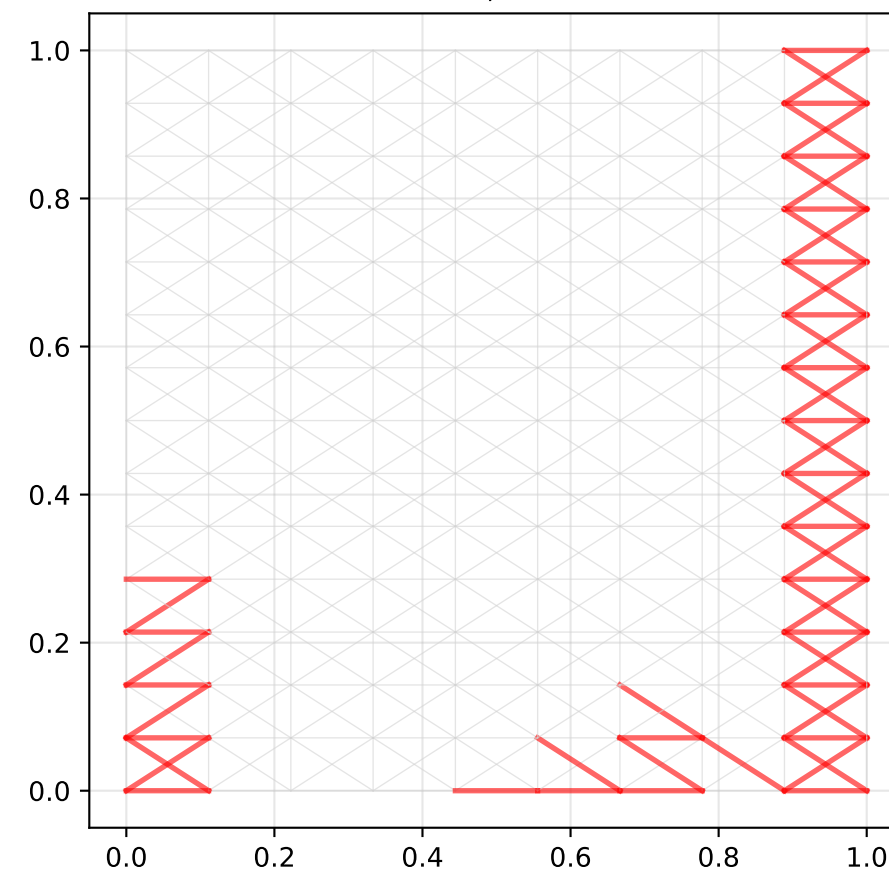
GGNI (Spectral) E=2.76, 61 cuts
