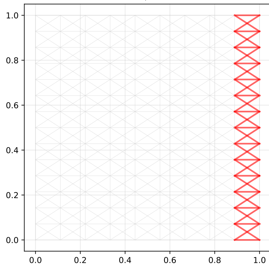
Gradient Descent E=2.40, 49 cuts
