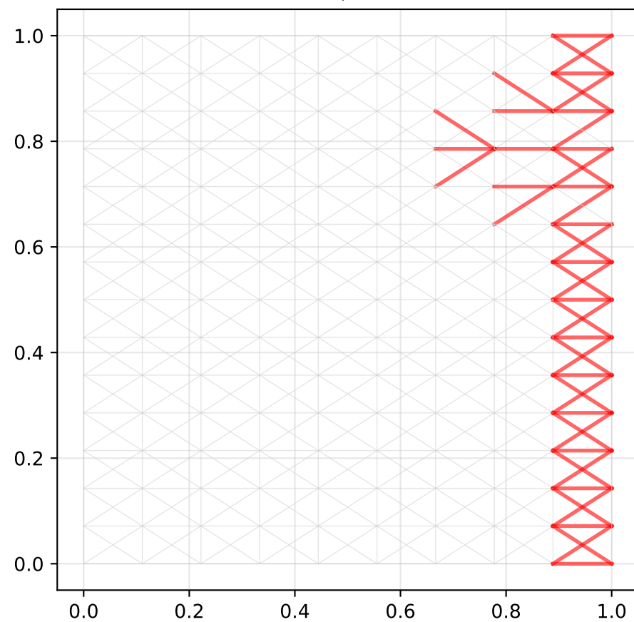
Gradient Descent E=2.40, 49 cuts
