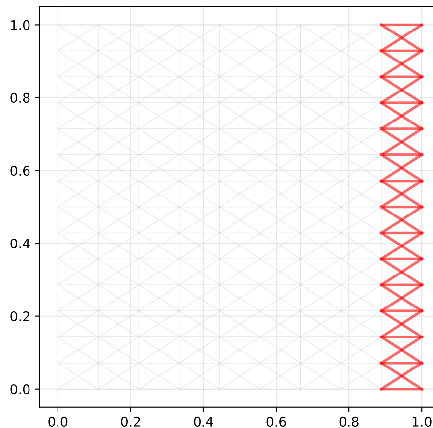
Simulated Annealing E=9.35, 149 cuts
