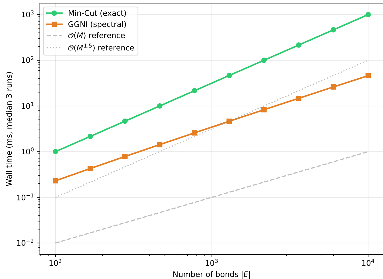
Empirical Scalability: n \times n Lattice
