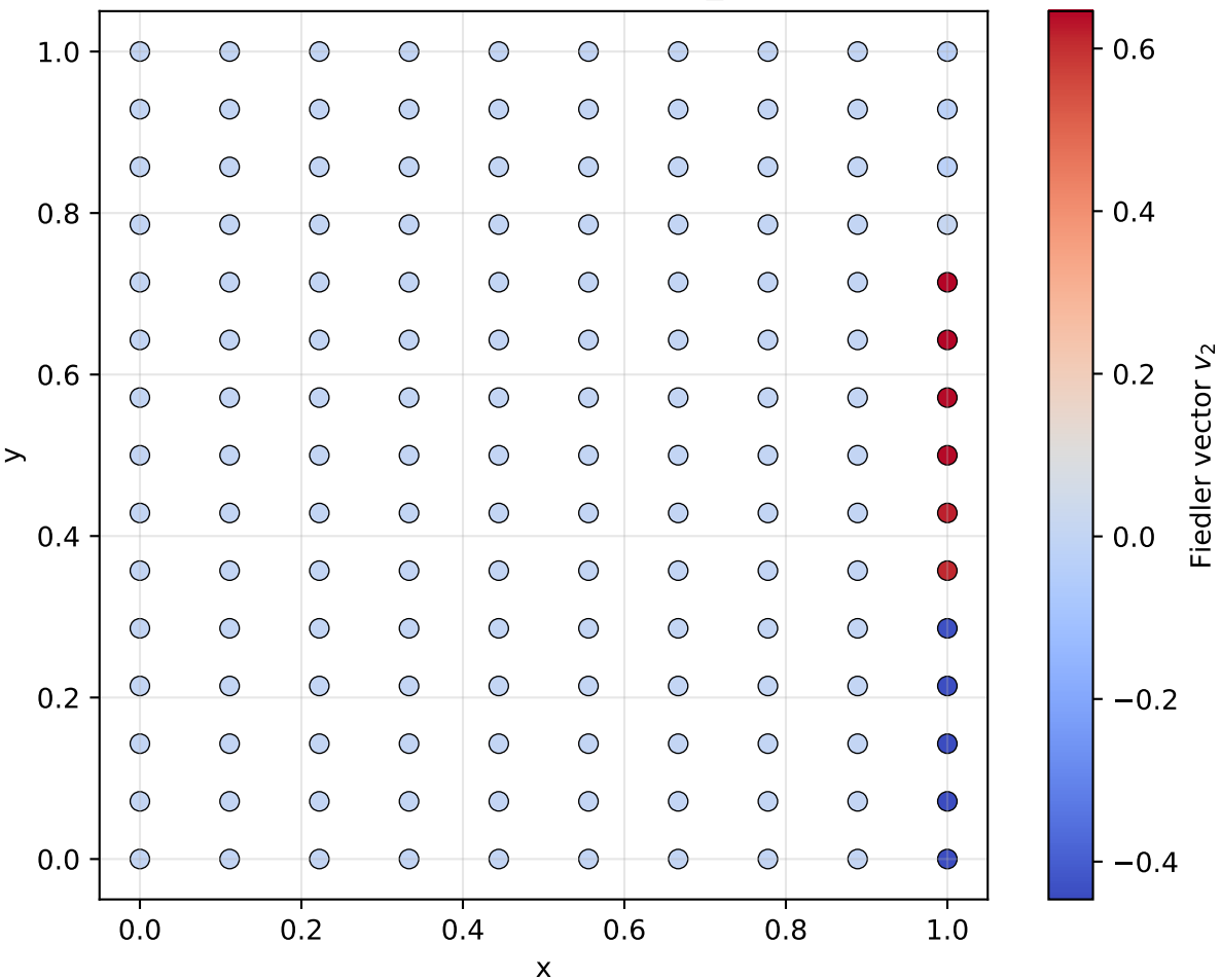
Fiedler vector v_2 on Geometria\_Transfinita
