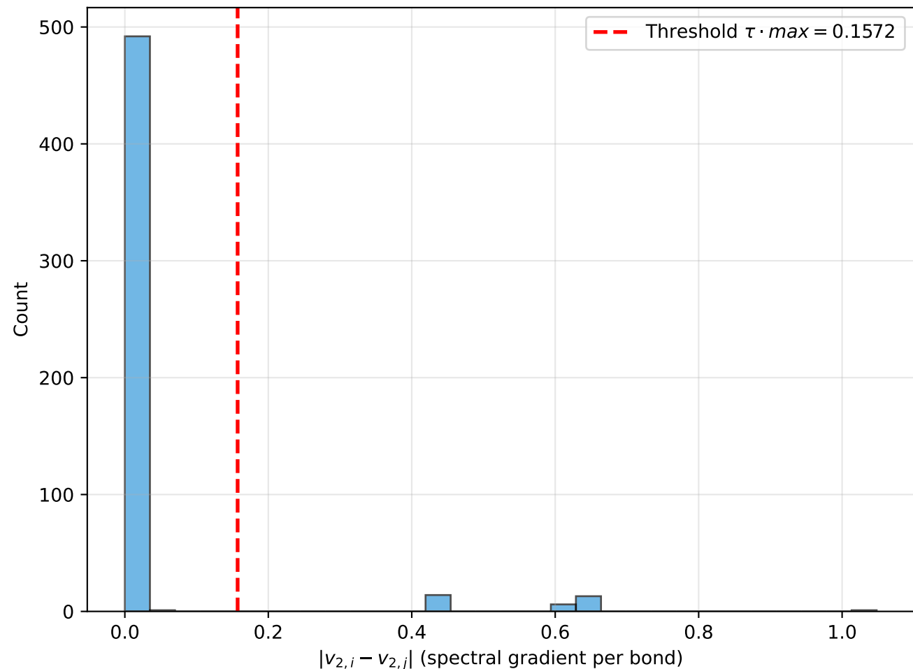
Spectral Gradient Distribution ( \beta=4.0 , \tau=0.15 ) 34 bonds above threshold
