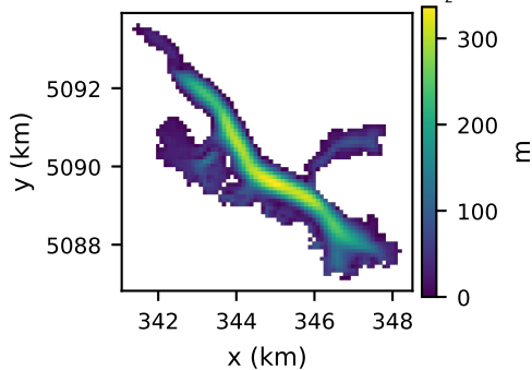
(a) Calibrated thickness H_{t_2}
