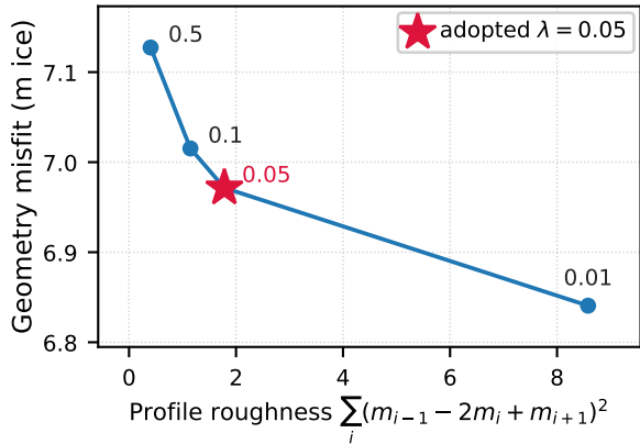
(a) Misfit vs smoothness
