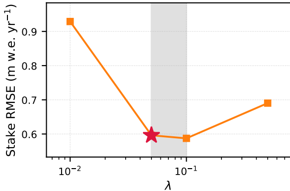
(b) Stake RMSE vs \lambda
