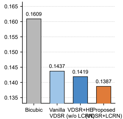
RMSE ↓
