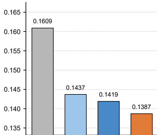
RMSE ↓
