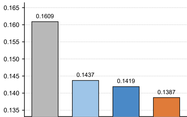
RMSE ↓
