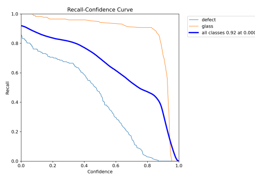
Figure 6: Recall Test
