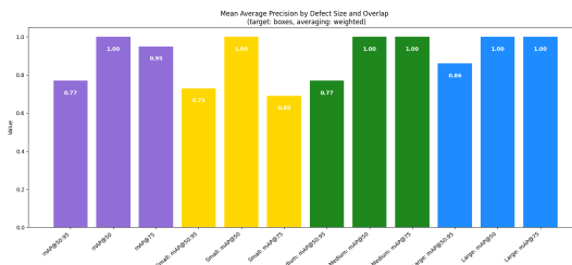
Figure 22: mAP Testing
