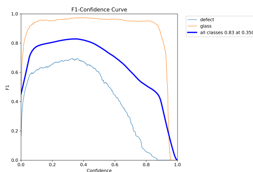
Figure 8: F1-Score Test
