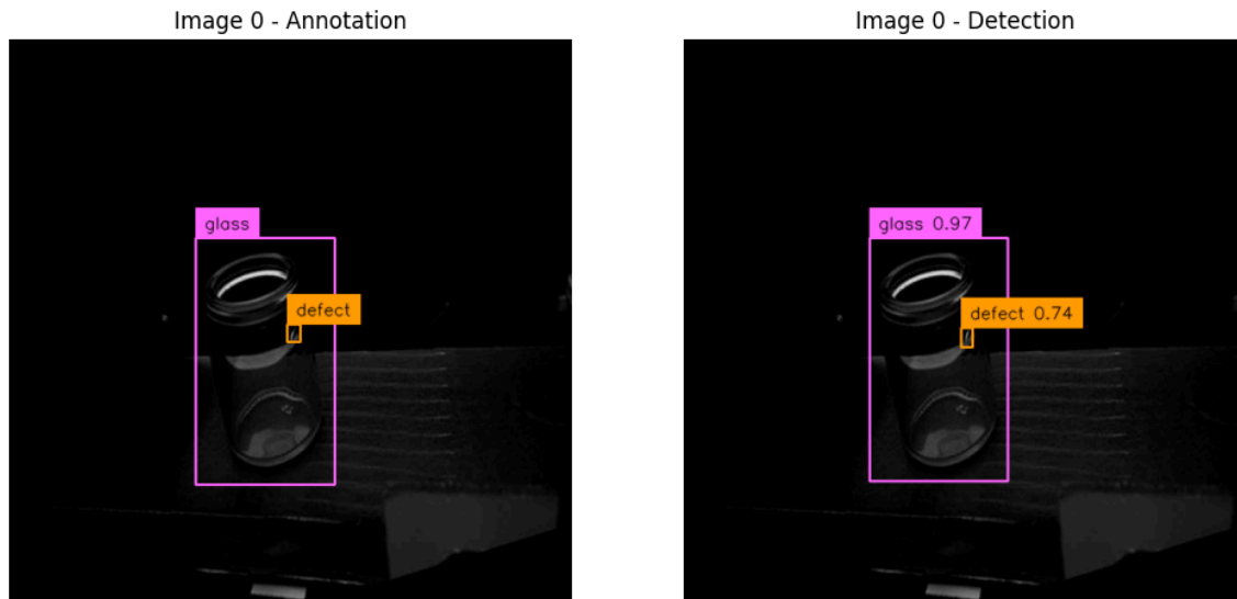
Figure 18: True Positive
