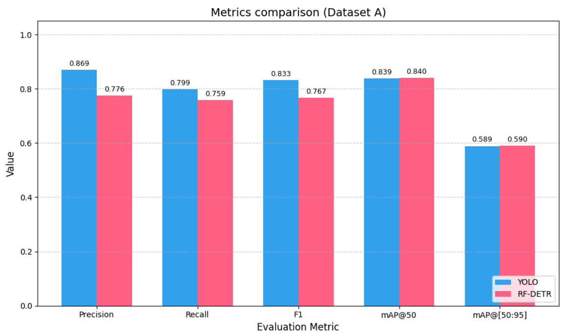
Figure 14: Visualization of Results for Dataset A
