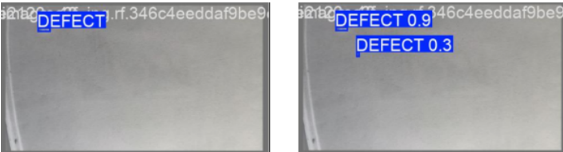
Figure 23: False Positive
