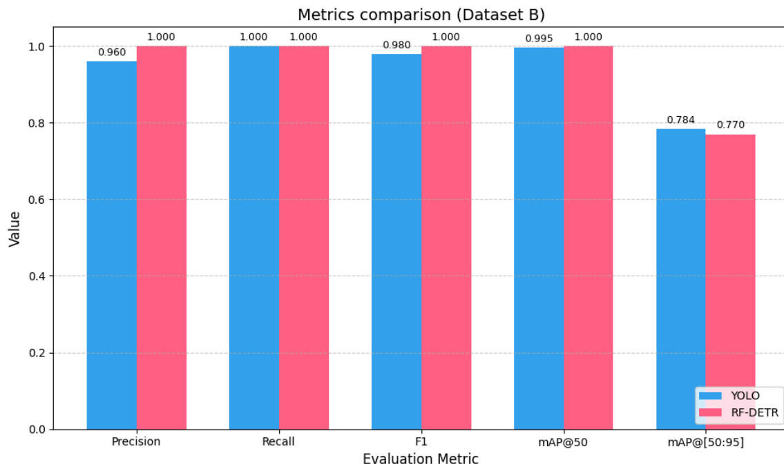
Figure 17: Visualization of Results for Dataset B
