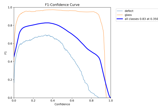
Figure 8: F1-Score Test
