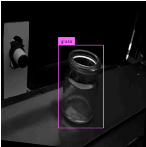
Figure 17: True Negative
