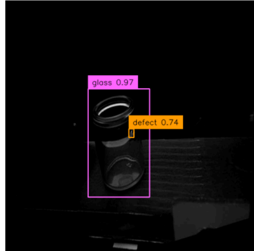
Figure 16: True Positive
