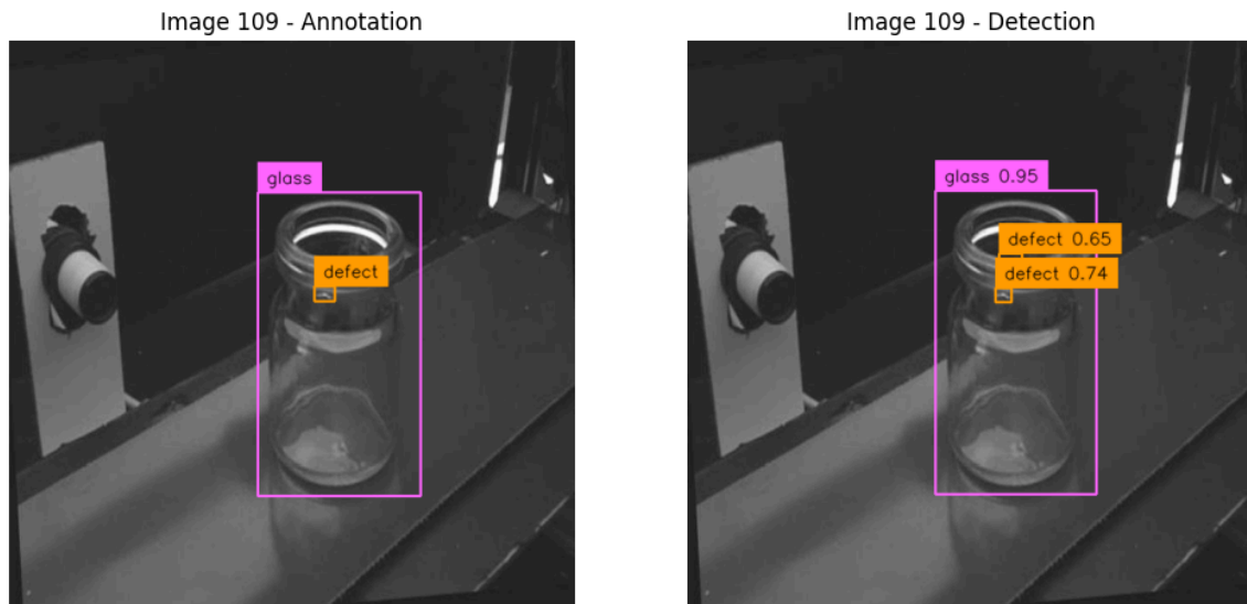
Figure 18: False Positive
