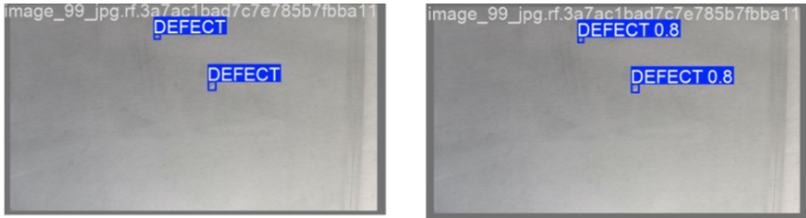
Figure 20: True Positive
