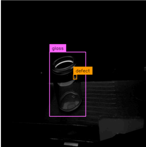
Figure 16: True Positive
