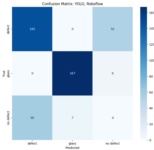
Figure 10: Confusion Matrix YOLO
