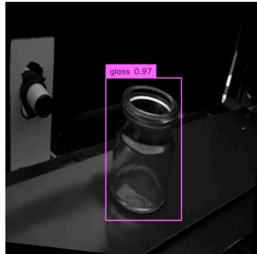
Figure 17: True Negative
